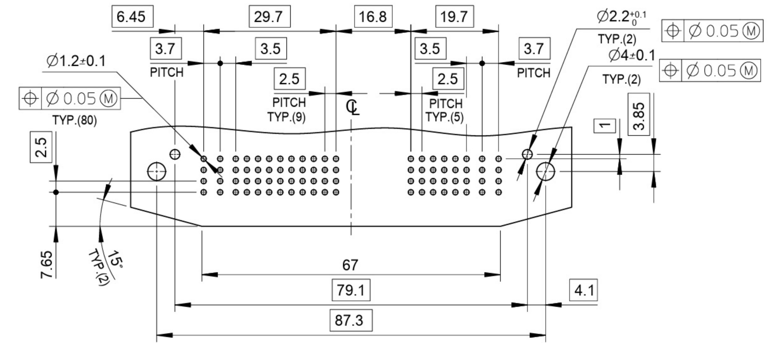
基板穴推奨寸法 (部品実装側) RECOMMENDED PCB LAYOUT (COMPONENT SIDE)
