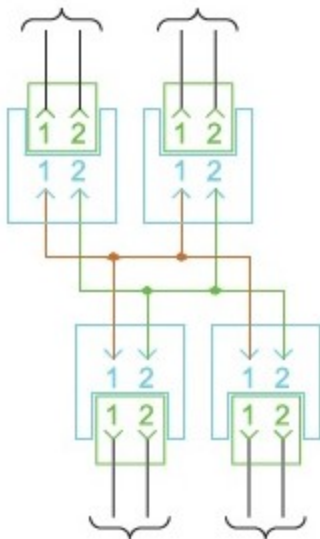
CIRCUIT DIAGRAM
