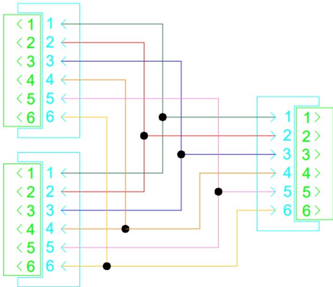
CIRCUIT DIAGRAM
