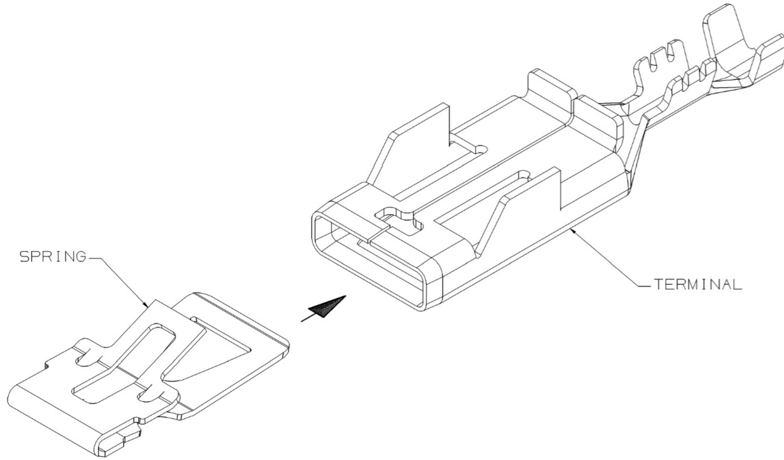
STANDARD ASSEMBLY SCALE 10:1
