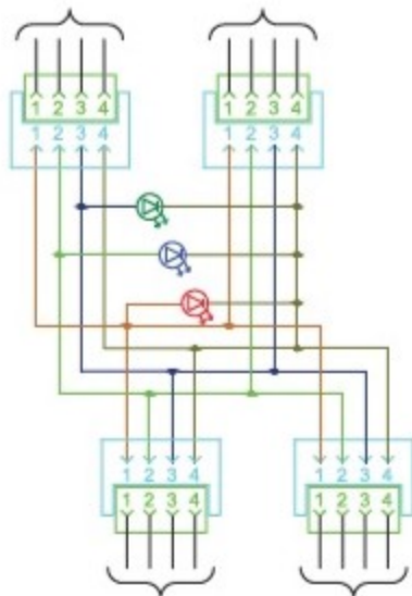
CIRCUIT DIAGRAM
