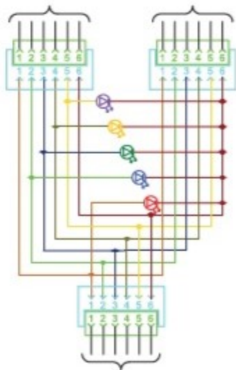
CIRCUIT DIAGRAM
