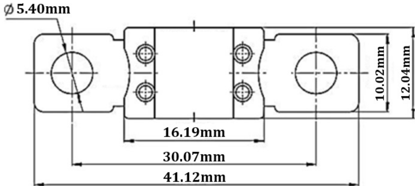
MEGA fuse
