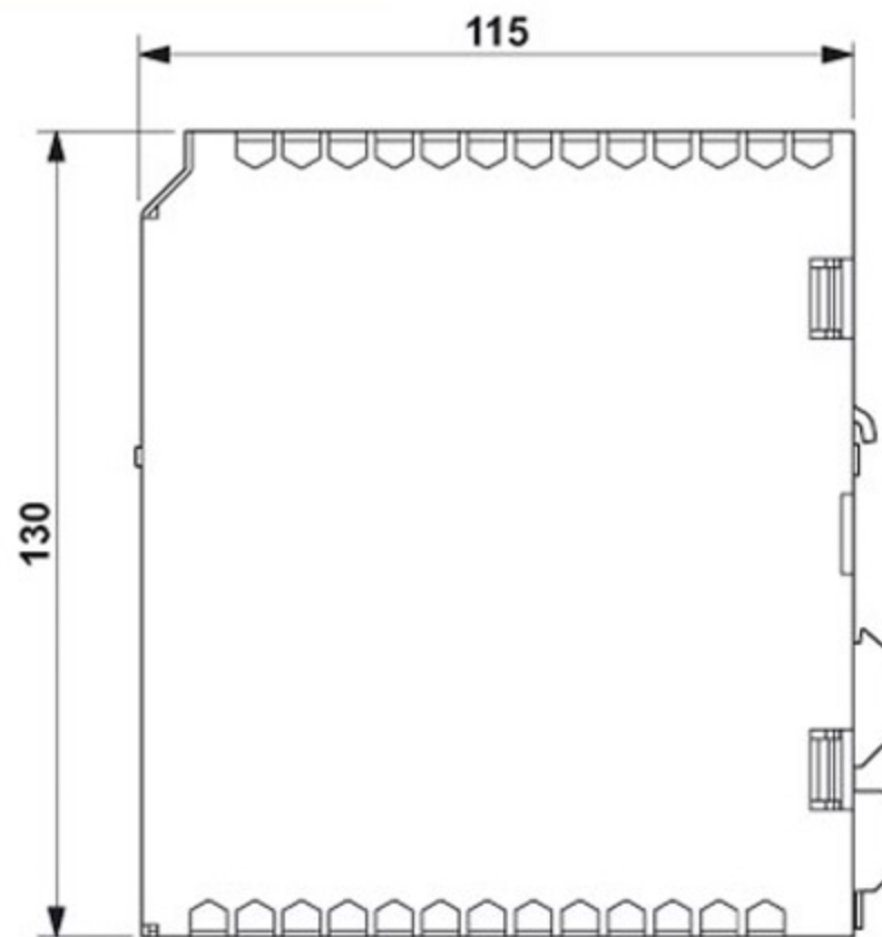
Dimensioned drawing
