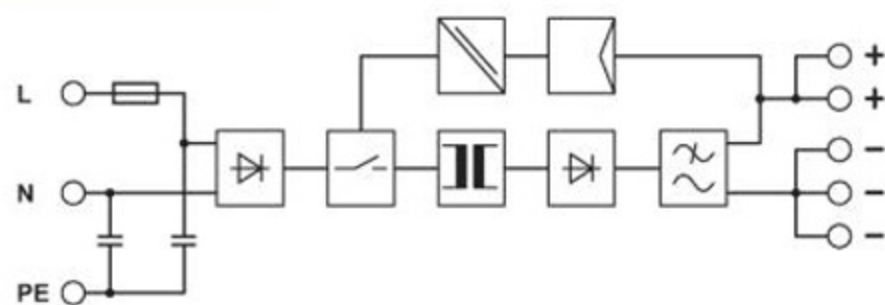
Block diagram
