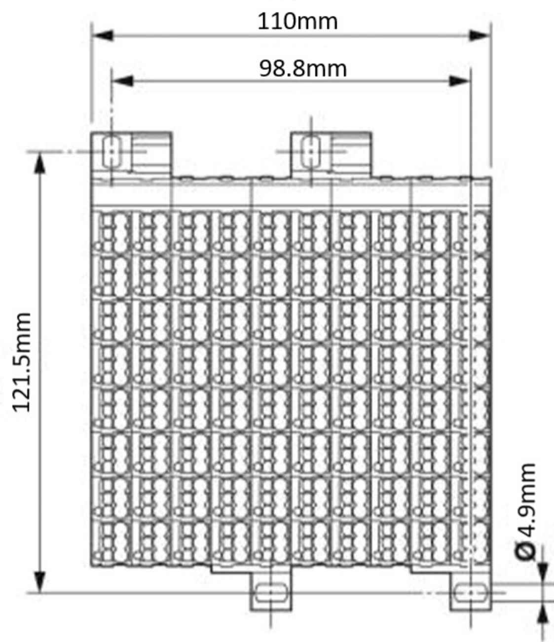
Dimensional drawing
