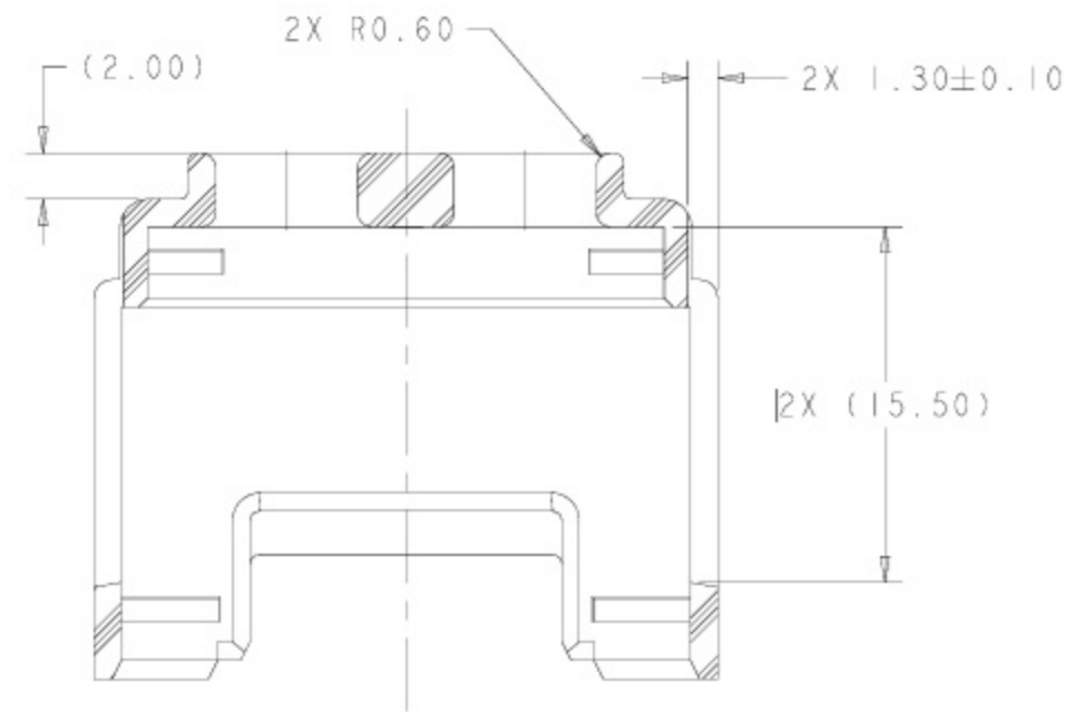
SECTION E-E REMOVED ROTATED CCW 90°
