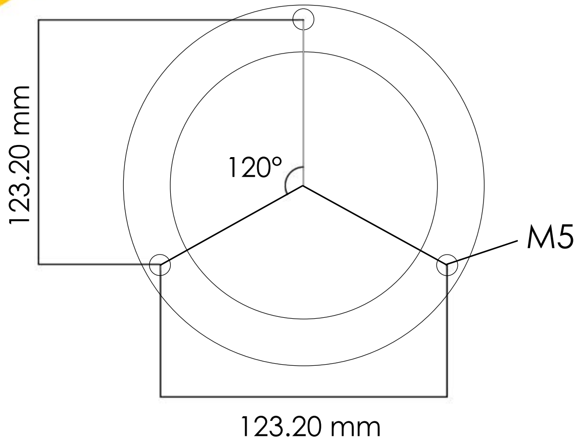
MOUNTING DIAGRAM
