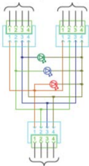
CIRCUIT DIAGRAM
