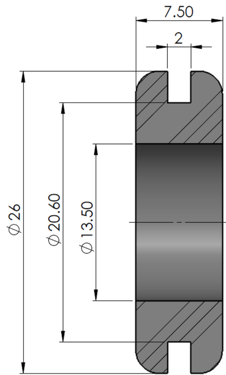
SECTION A-A SCALE 3.5 : 1
