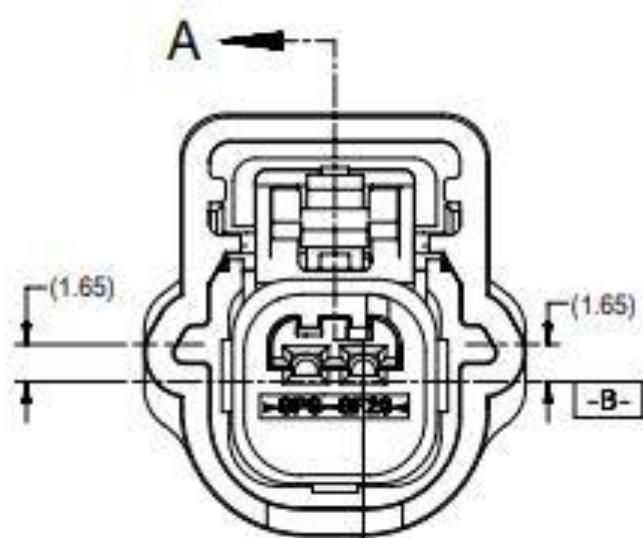
A FRONT VIEW POLARIZATION A
