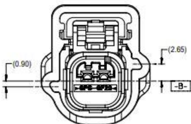
A FRONT VIEW POLARIZATION A
